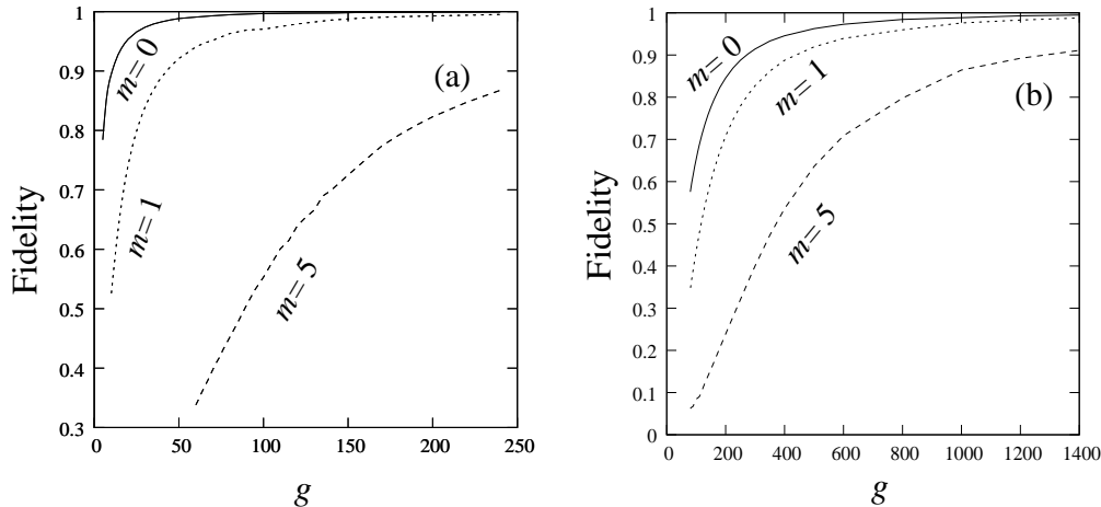
FIG. 3: Overlap fidelity vs. g for an initial state |(\alpha, m); 0\rangle , with \gamma = 1 and (a) \nu = 1 and (b) \nu = 5 .
